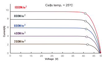
I-V curve
